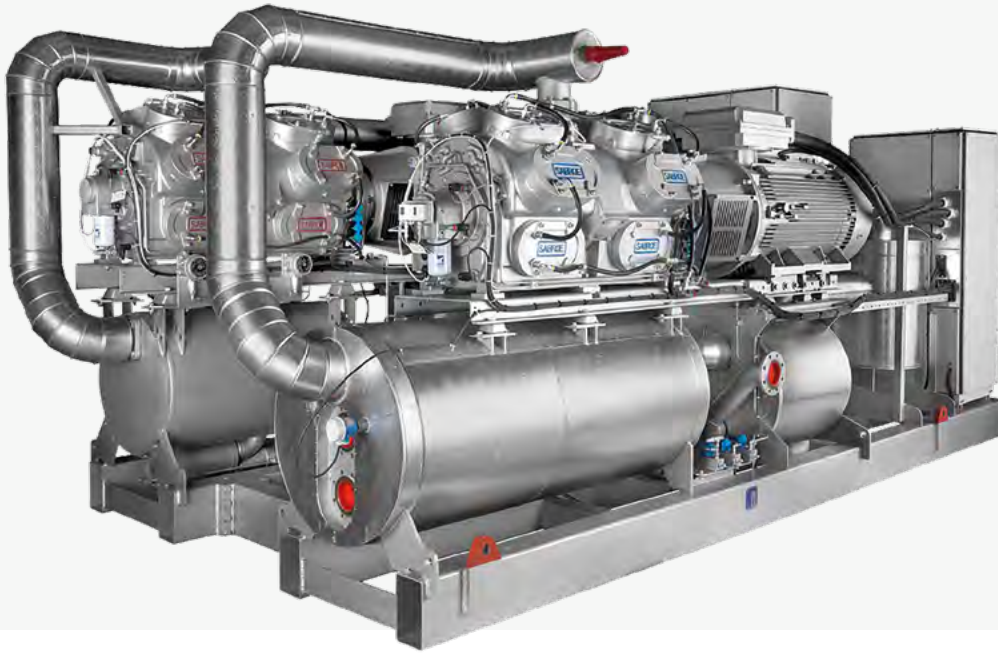
DualPAC heat pump unit with panel-mounted UniSAB systems controllers
